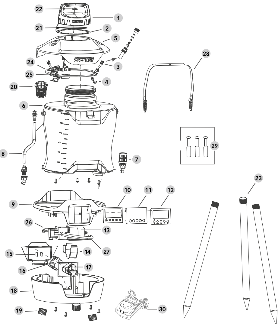
Serbatoio 4 L Tanque 4 L Tank 4 L Art. 410/1
