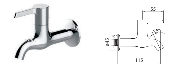
Grifo de pared. Wall mounted single tap. Robinet
