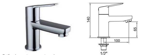
Grifo de repisa con aireador Deck mounted single basin tap, with aerator Robinet, aérateur
