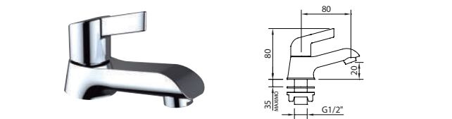
Grifo de repisa con aireador Deck mounted single basin tap, with aerator Robinet, aérateur
