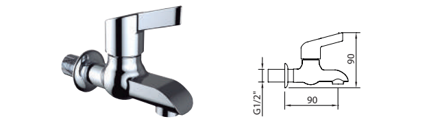
Grifo mural con aireador. Wall single basin tap, with aerator. Robinet, aérateur
