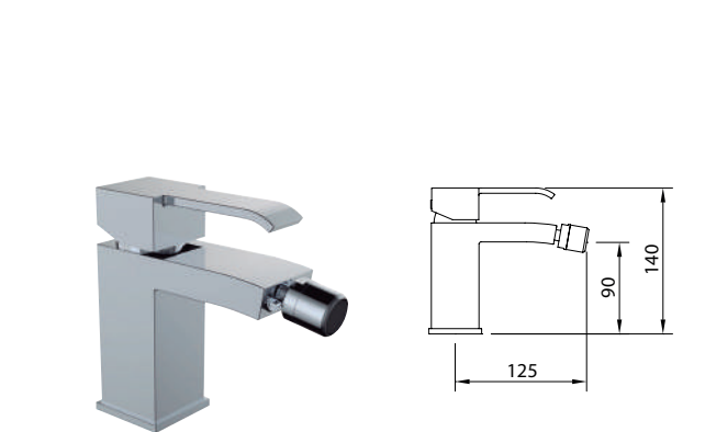
Mezclador con aireador a rótula, flexibles M-10 3/8" x 420 mm. Mixer, swivel aerator, flexible hoses M-10 3/8" x 420 mm. Mitigeur bidet, aérateur rotule, raccords flexibles M-10 3/8" x 420 mm
