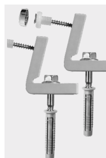
Tornillos TI 5 Ref. 0140564080 Packaging Bolsa 25 uds/caja PVP: 7,18 € Inodoro / Bidé Horizontal
